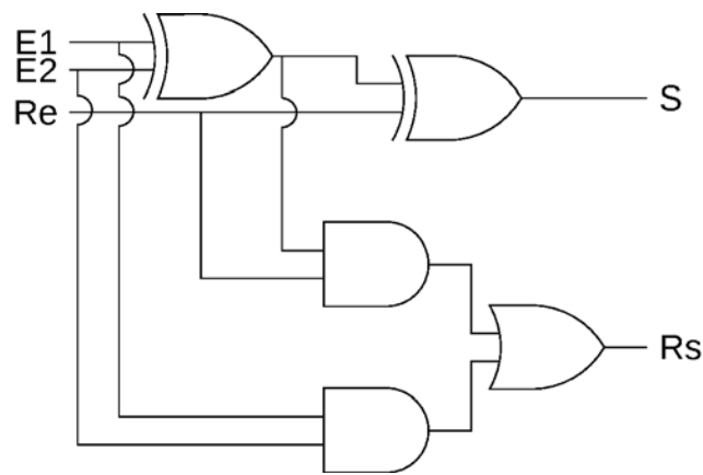
Figure 3. Circuit logique
